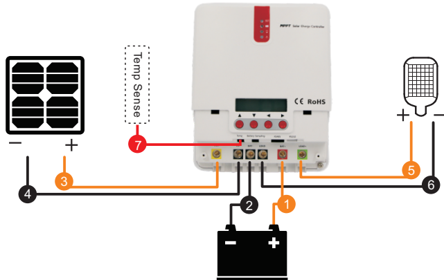
Figure 2-3 Wiring
